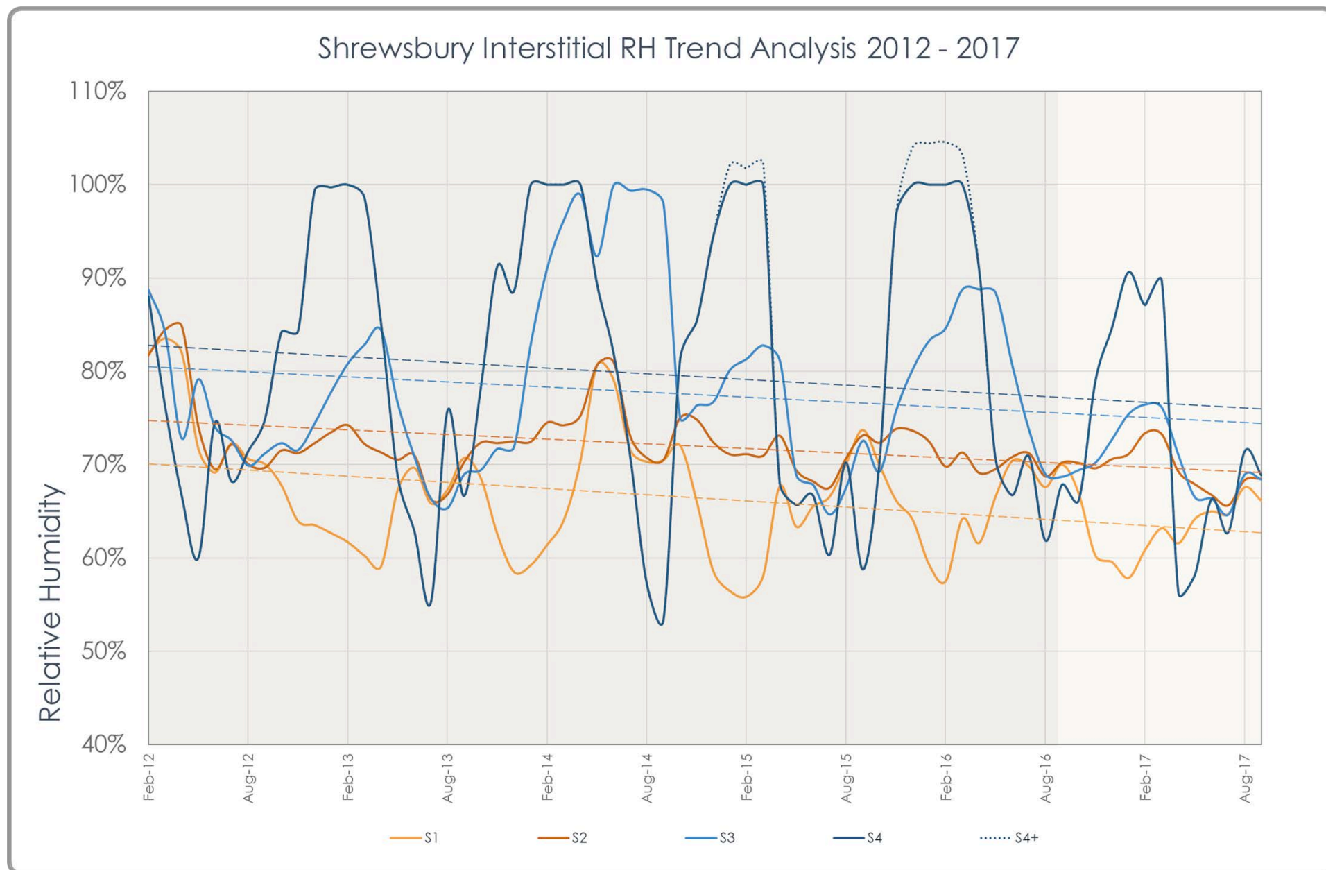
Figure 49. Relative humidity trends over time, Shrewsbury 2012-2017.
