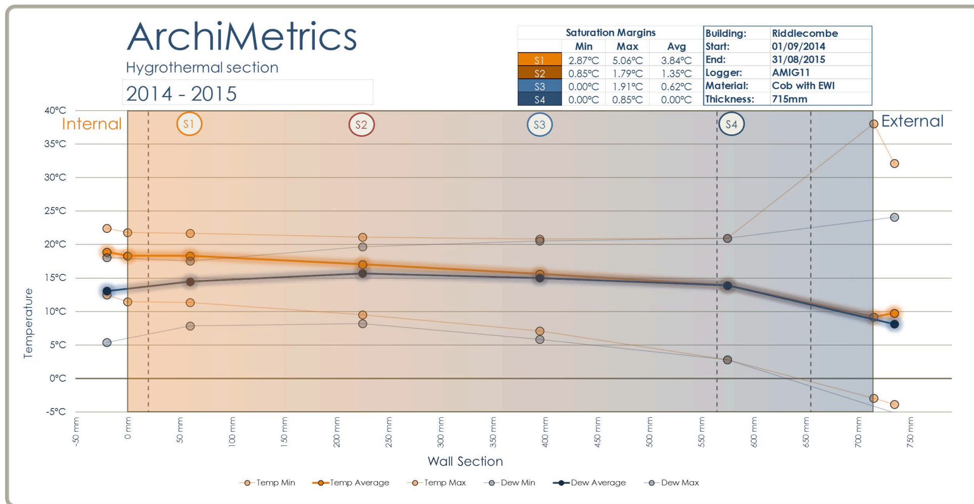
Figure 44. Hygrothermal section, The Firs, Riddlecombe, 2014-2015.
