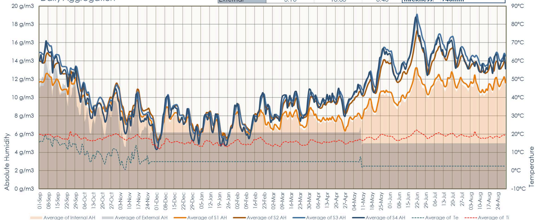
Figure 25. Absolute humidity over time, Mill House, Drewsteignton 2016-2017.
