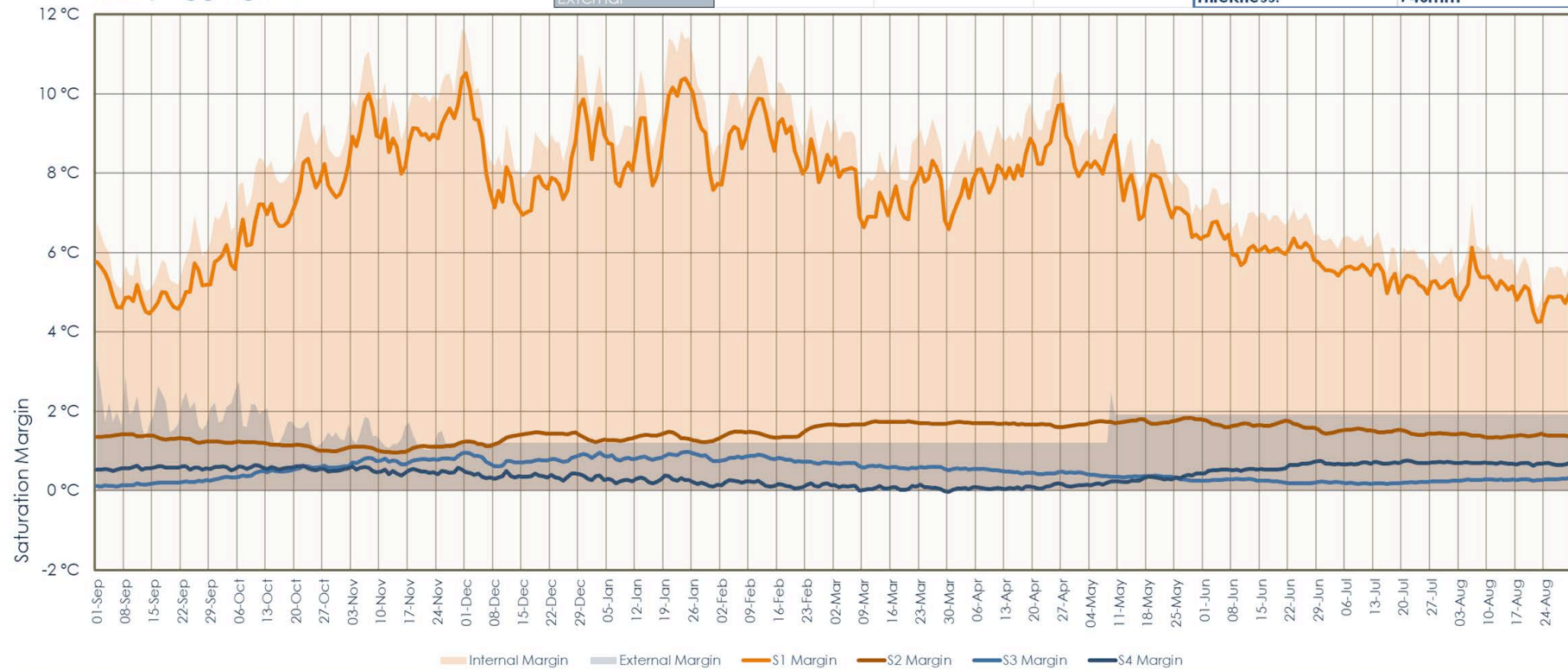
Figure 27. Saturation margin over time, Mill House, Drewsteignton, 2016-2017.
