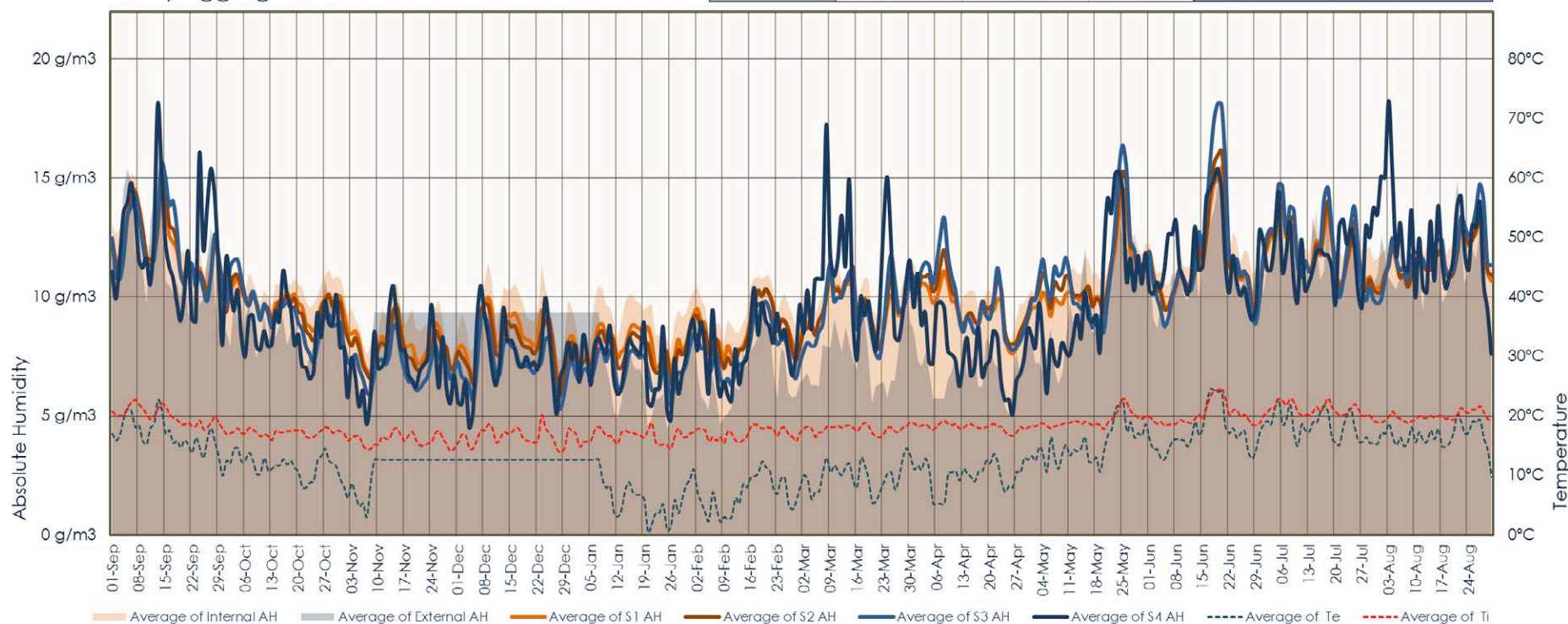
Figure 9. Absolute humidity over time, daily aggregation, Abbeyforegate, Shrewsbury 2016-2017.
