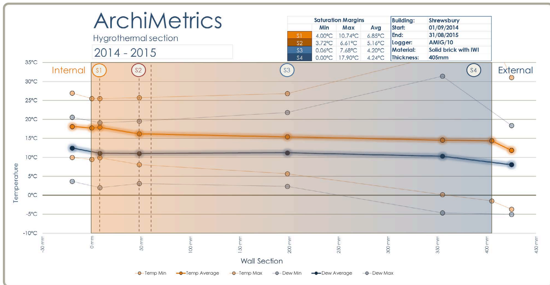
Figure 14. Hygrothermal section, Abbeyforegate, Shrewsbury 2014–2015 (capped).
