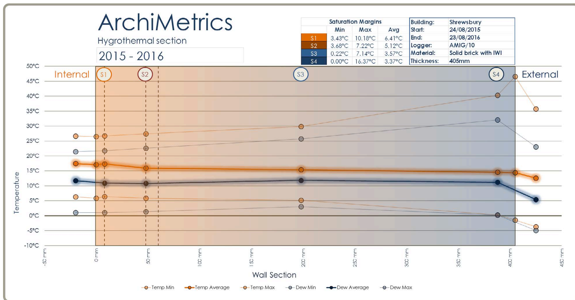
Figure 13. Hygrothermal section, Abbeyforegate, Shrewsbury 2015–2016 (capped).
