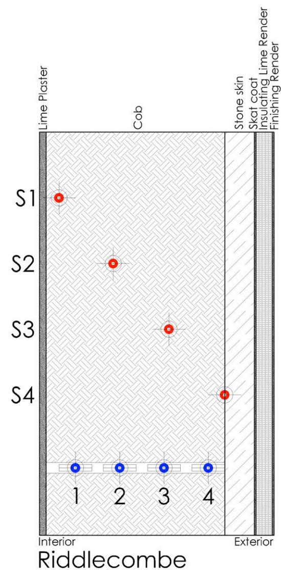
Figure 38. Position of sensors through wall section, Riddlecombe.
