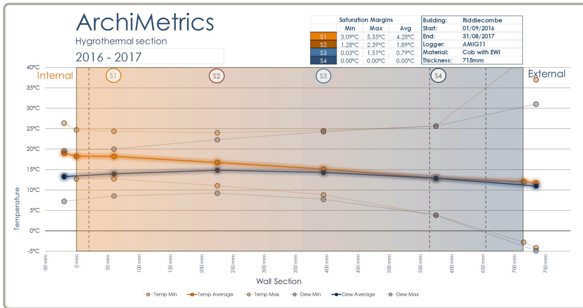
Figure 42. Hygrothermal section, The Firs, Riddlecombe, 2016-2017.
