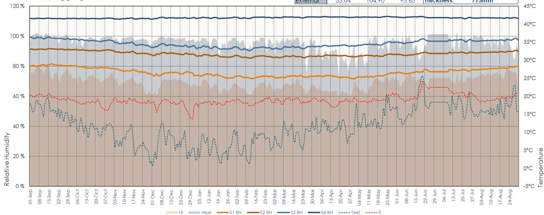
Figure 39. Relative humidity over time, The Firs, Riddlecombe 2016-2017.
