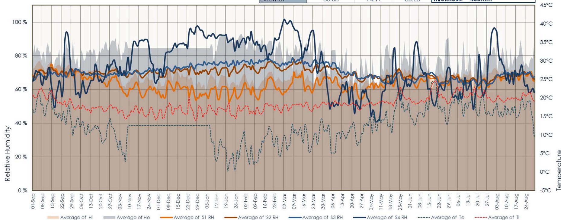
Figure 5. Relative humidity over time, daily aggregation, Abbeyforegate, Shrewsbury 2016-2017. (Ti = Internal temperature, Te = External temperature, Hi = Internal RH, He = External RH.)
