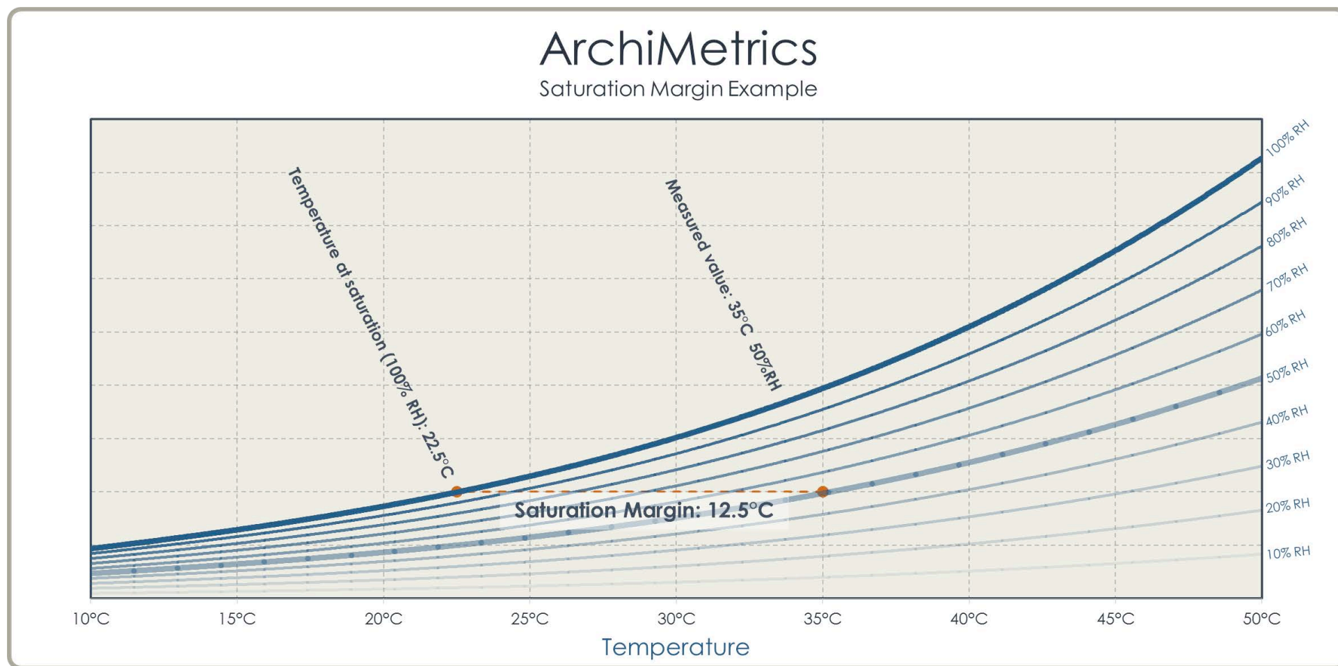
Figure 1. Illustration of saturation margin principle
