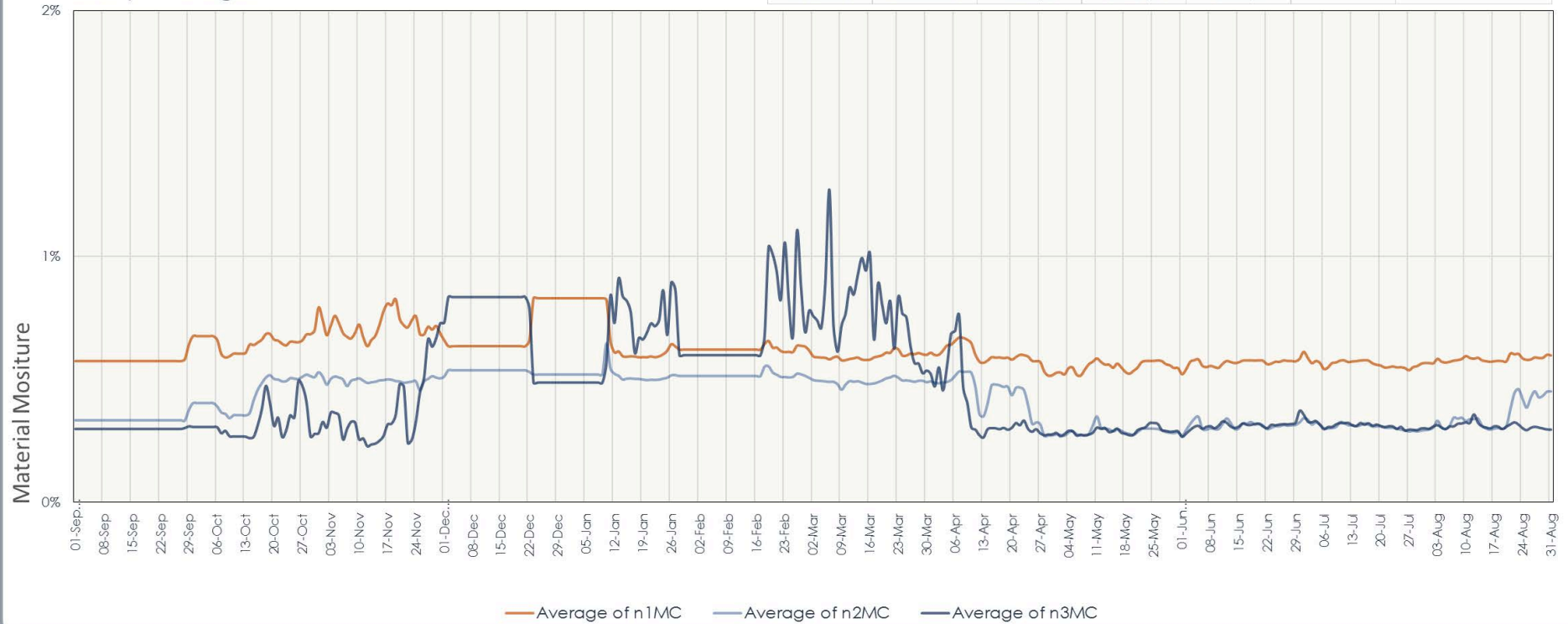
Figure 19. Material moisture content over time, Abbeyforegate, Shrewsbury 2014-2015.
