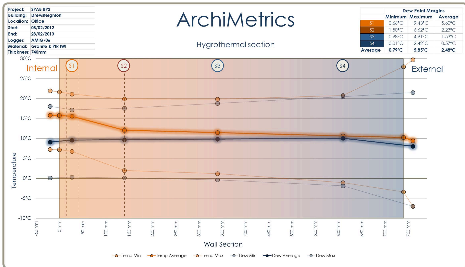
Figure 32. Hygrothermal section, Mill House, Drewsteignton, 2012-2013.
