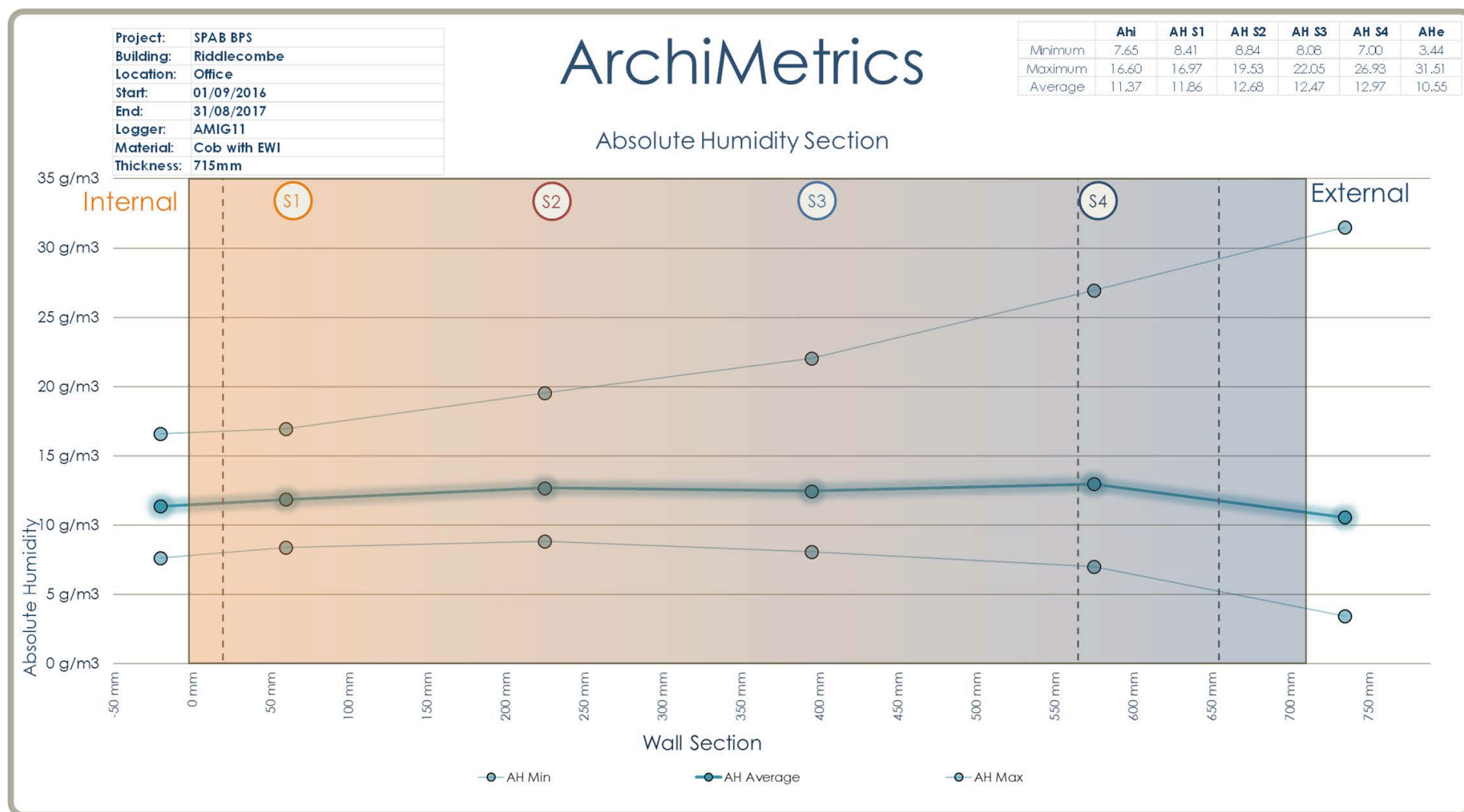
Figure 56. Absolute humidity average section, Riddlecombe, 2016-2017.
