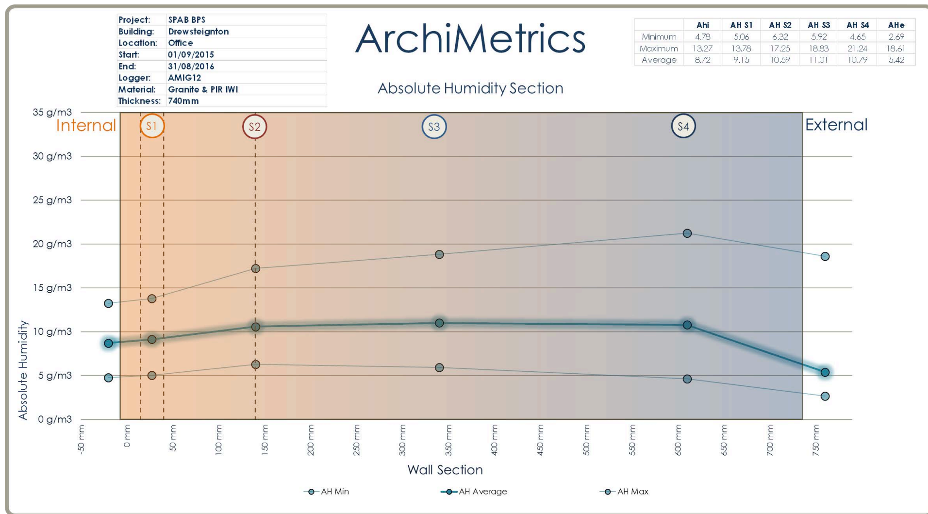
Figure 55.. Absolute humidity average section, Drewsteignton, 2015 -2016.
