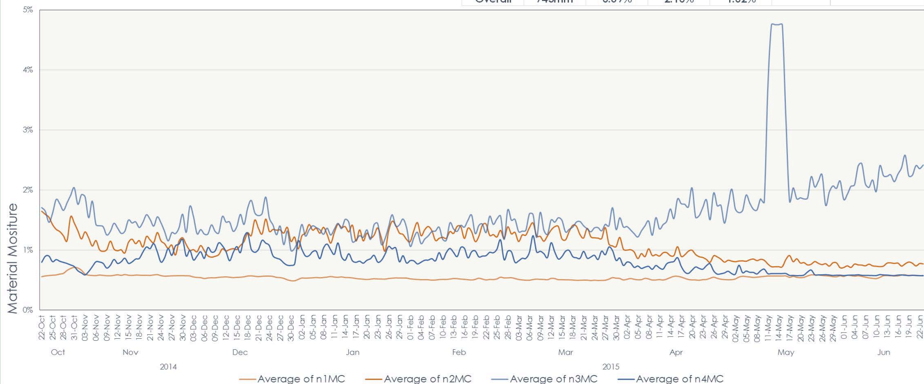
Figure 35. Material moisture content over time, Mill House, Drewsteignton, 2014-2015.
