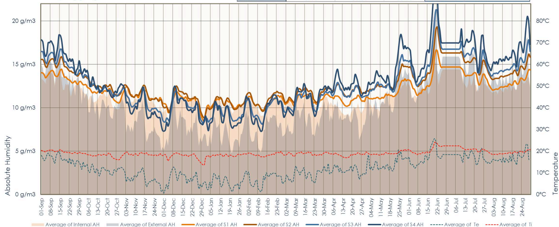
Figure 40. Absolute humidity over time, The Firs, Riddlecombe, 2016-2017.
