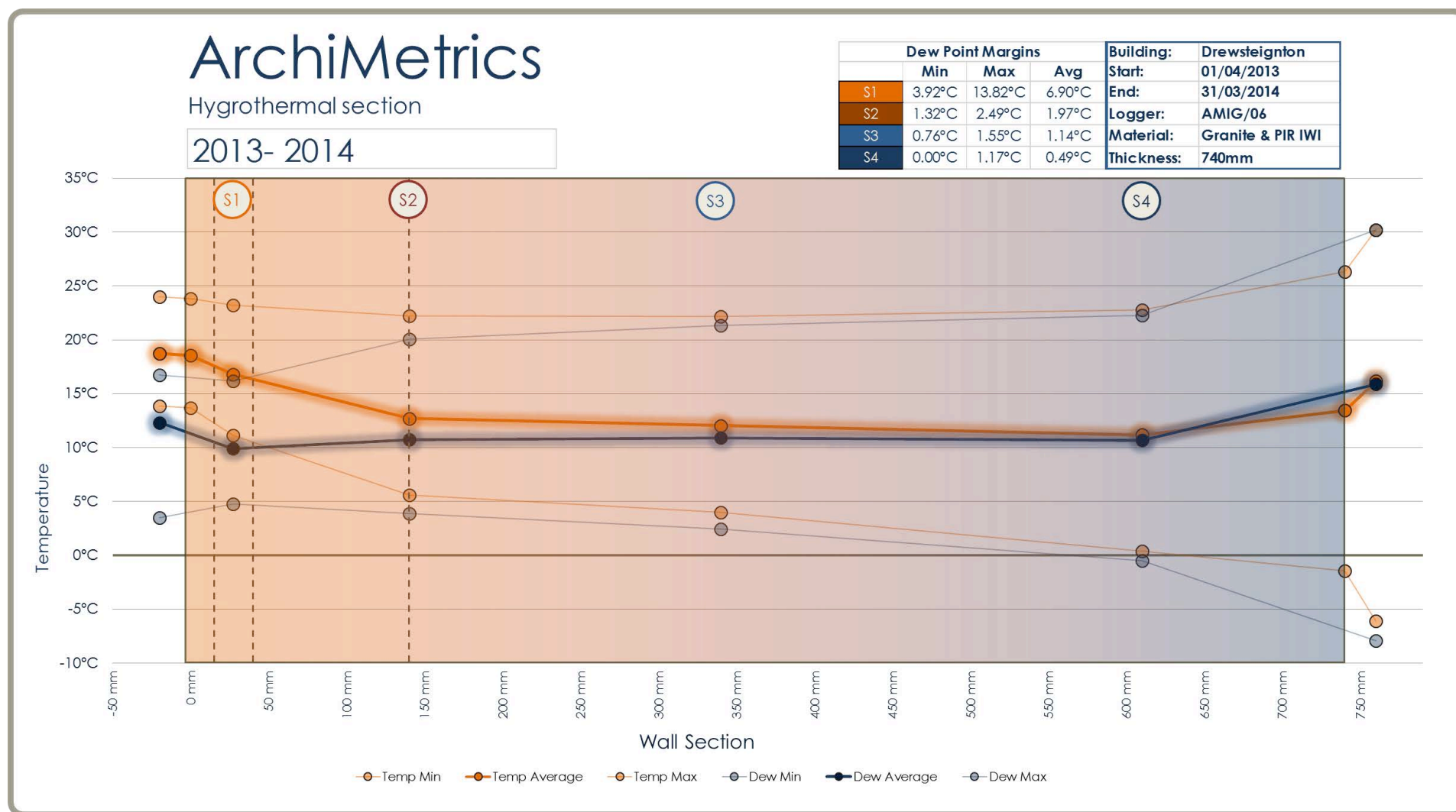
Figure 31. Hygrothermal section, Mill House, Drewsteignton, 2013-2014.
