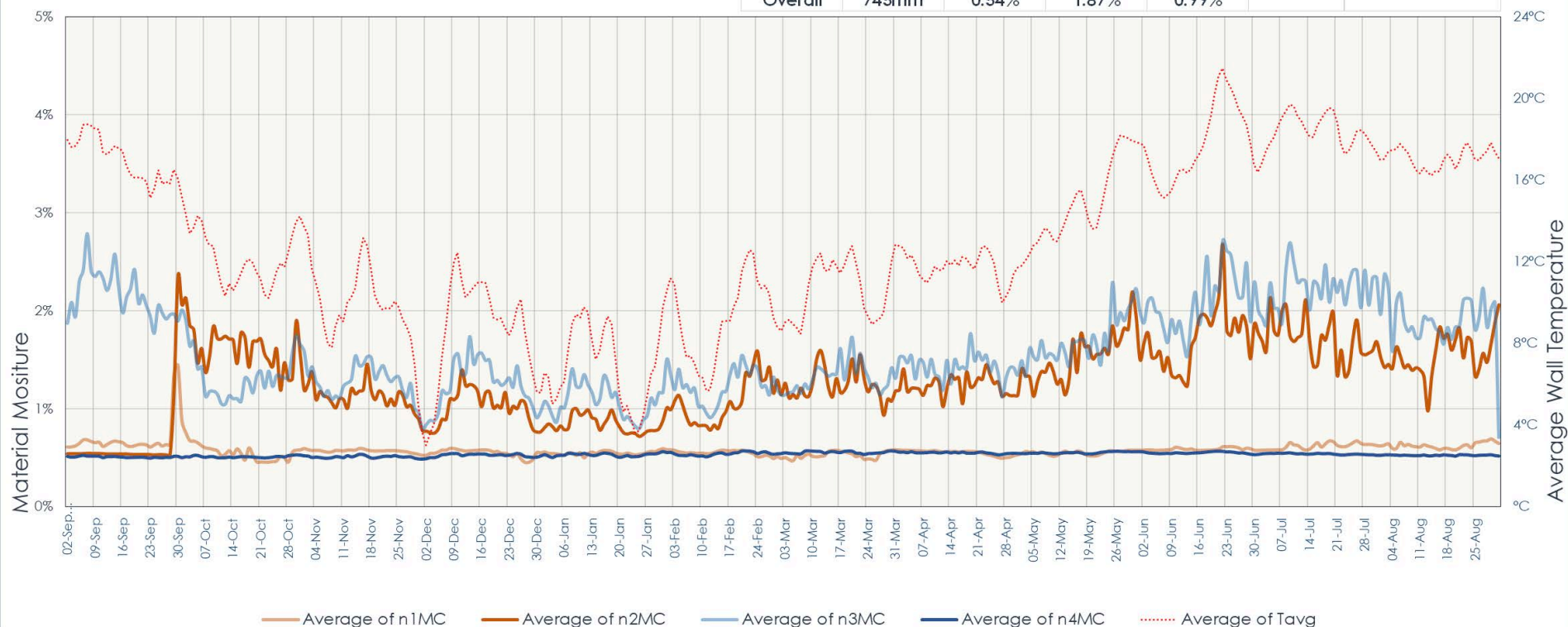
Figure 33. Material moisture content over time, Mill House, Drewsteignton, 2016-2017.
