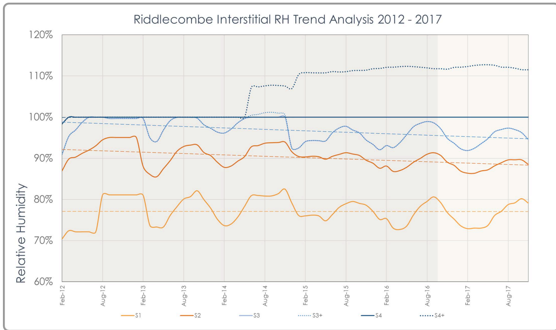
Figure 51. Relative humidity trends over time, Riddlecombe, 2012-2017.
