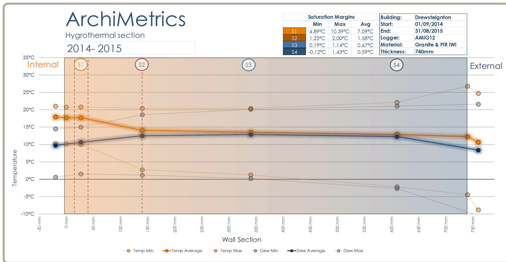
Figure 30. Hygrothermal section, Mill House, Drewsteignton, 2014–2015 .
