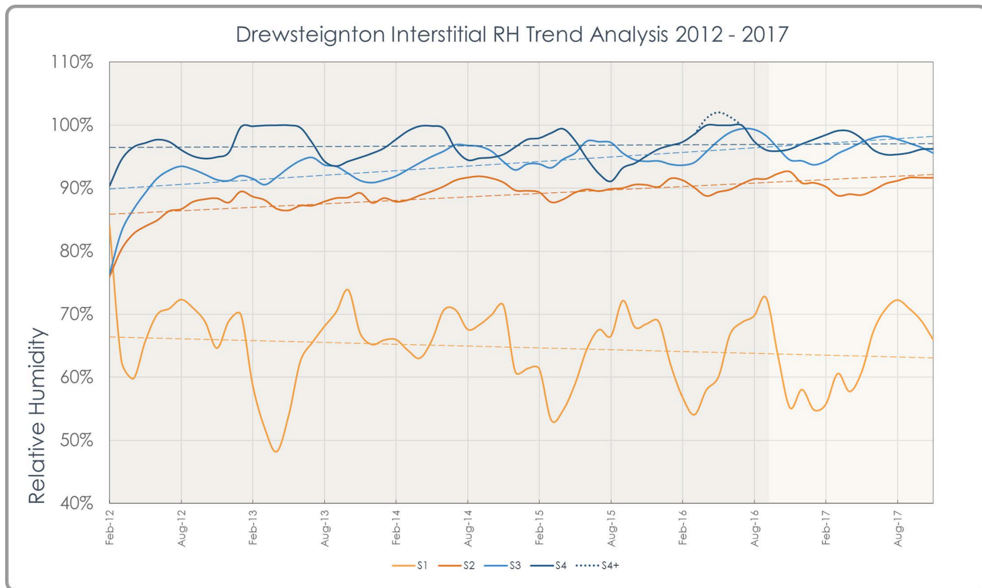
Figure 50. Relative humidity trends over time, Drewsteignton 2012–2017.
