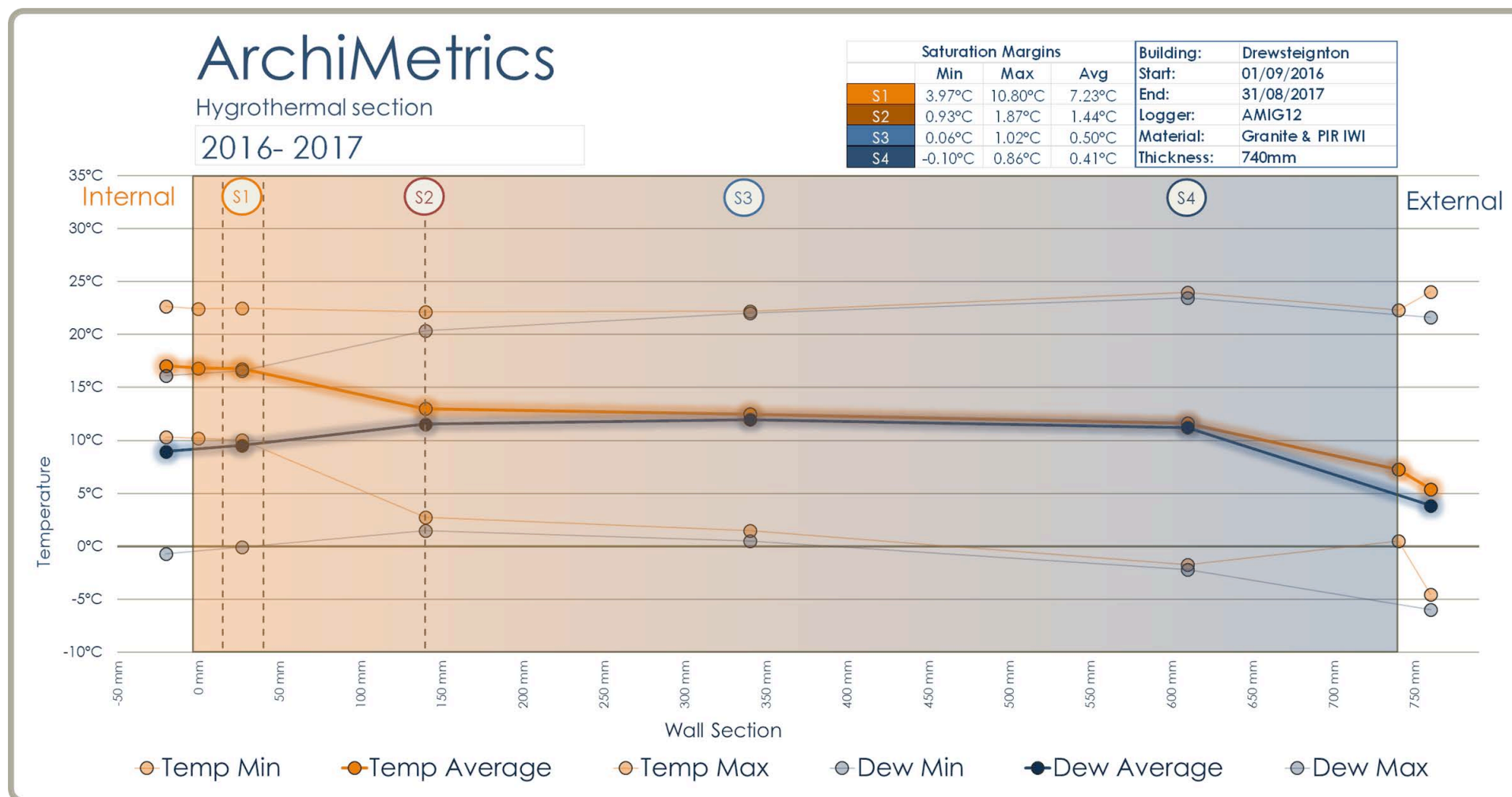
Figure 28. Hygrothermal section, Mill House, Drewsteignton, 2016–2017 (capped).
