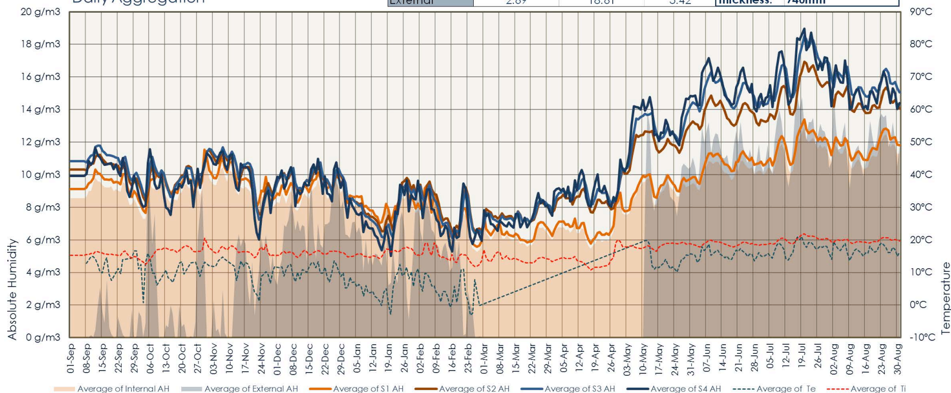
Figure 26. Absolute humidity over time, Mill House, Drewsteignton 2015-2016.
