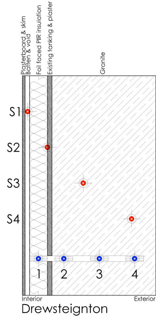
Figure 22. Position of wall sensors through section, Drewsteignton – red IHGM, blue material moisture
