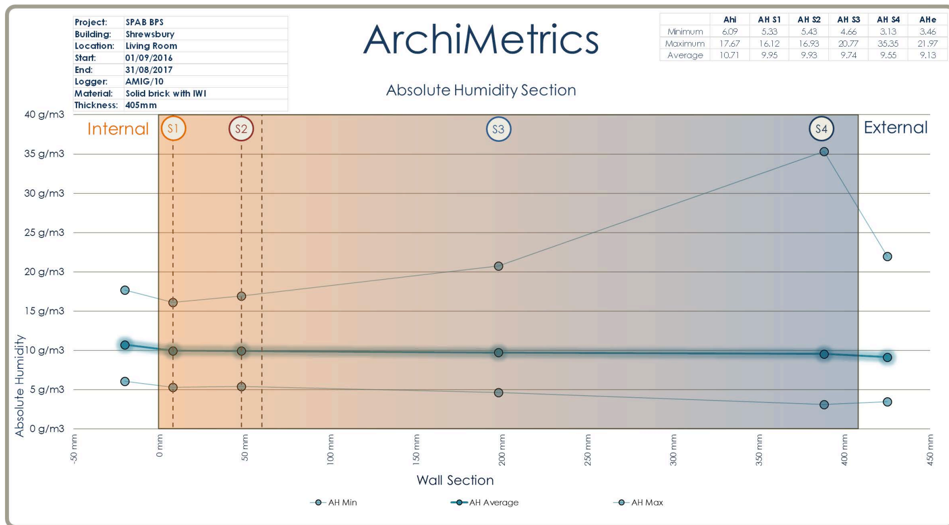
Figure 52. Absolute humidity average Section, Shrewsbury, 2016-2017.
