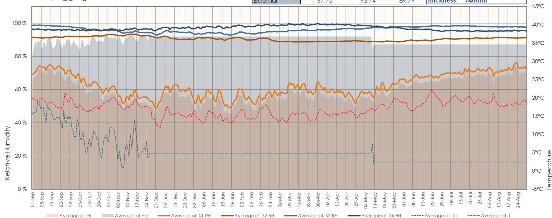
Figure 23. Relative humidity over time, daily aggregation, Mill House, Drewsteignton, 2016-2017.
