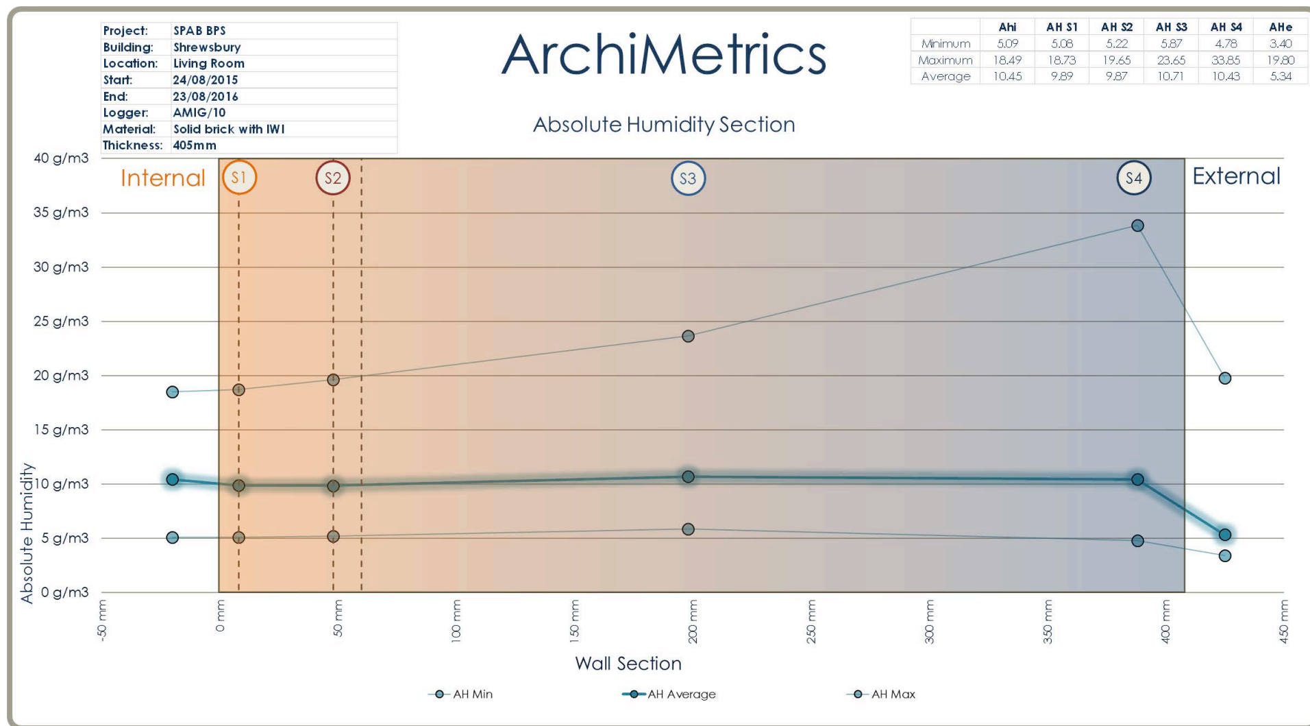
Figure 53. Absolute humidity average section, Shrewsbury, 2015 -2016.
