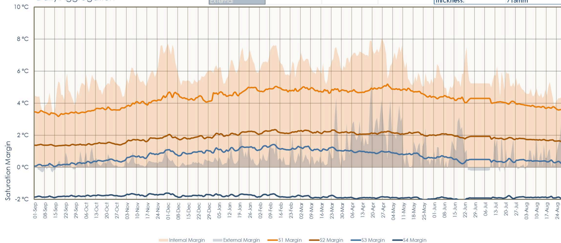
Figure 41. Saturation margin over time, The Firs, Riddlecombe, 2016-2017.
