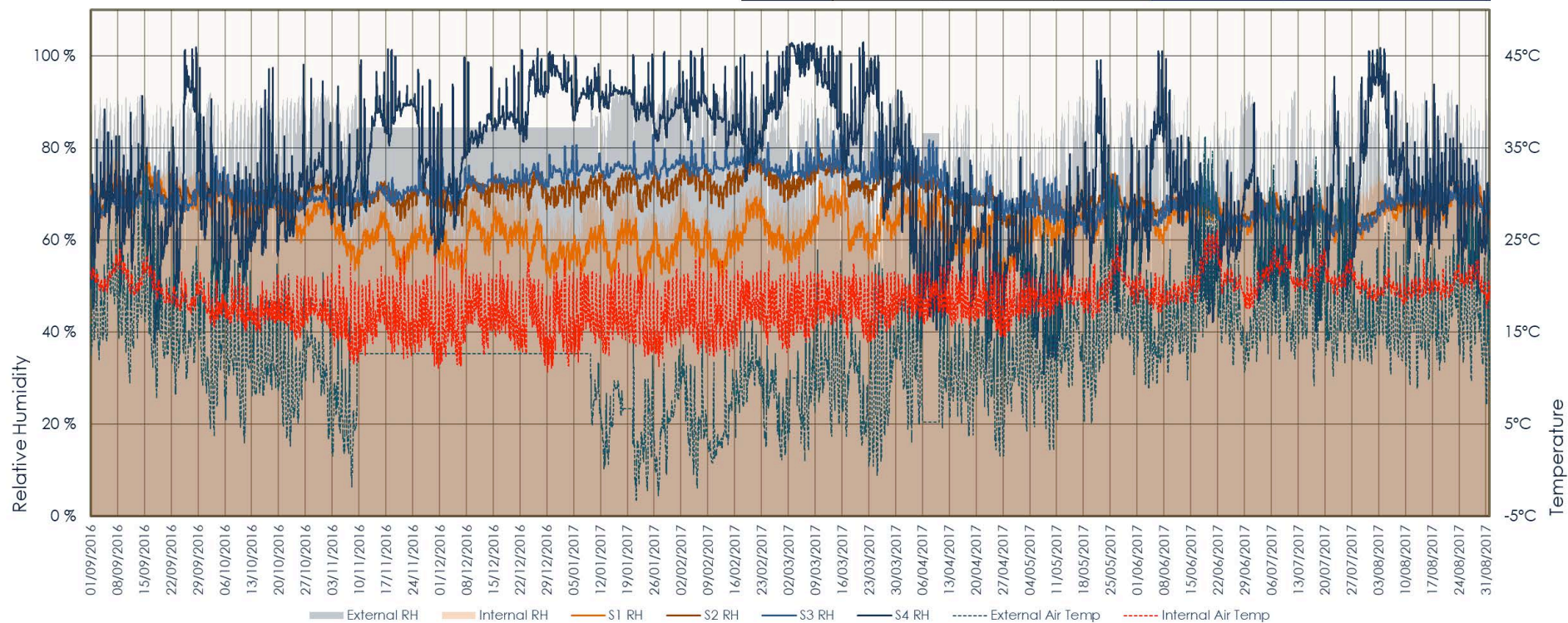
Figure 6. Relative humidity over time, full resolution, Abbeyforegate, Shrewsbury 2016-2017
