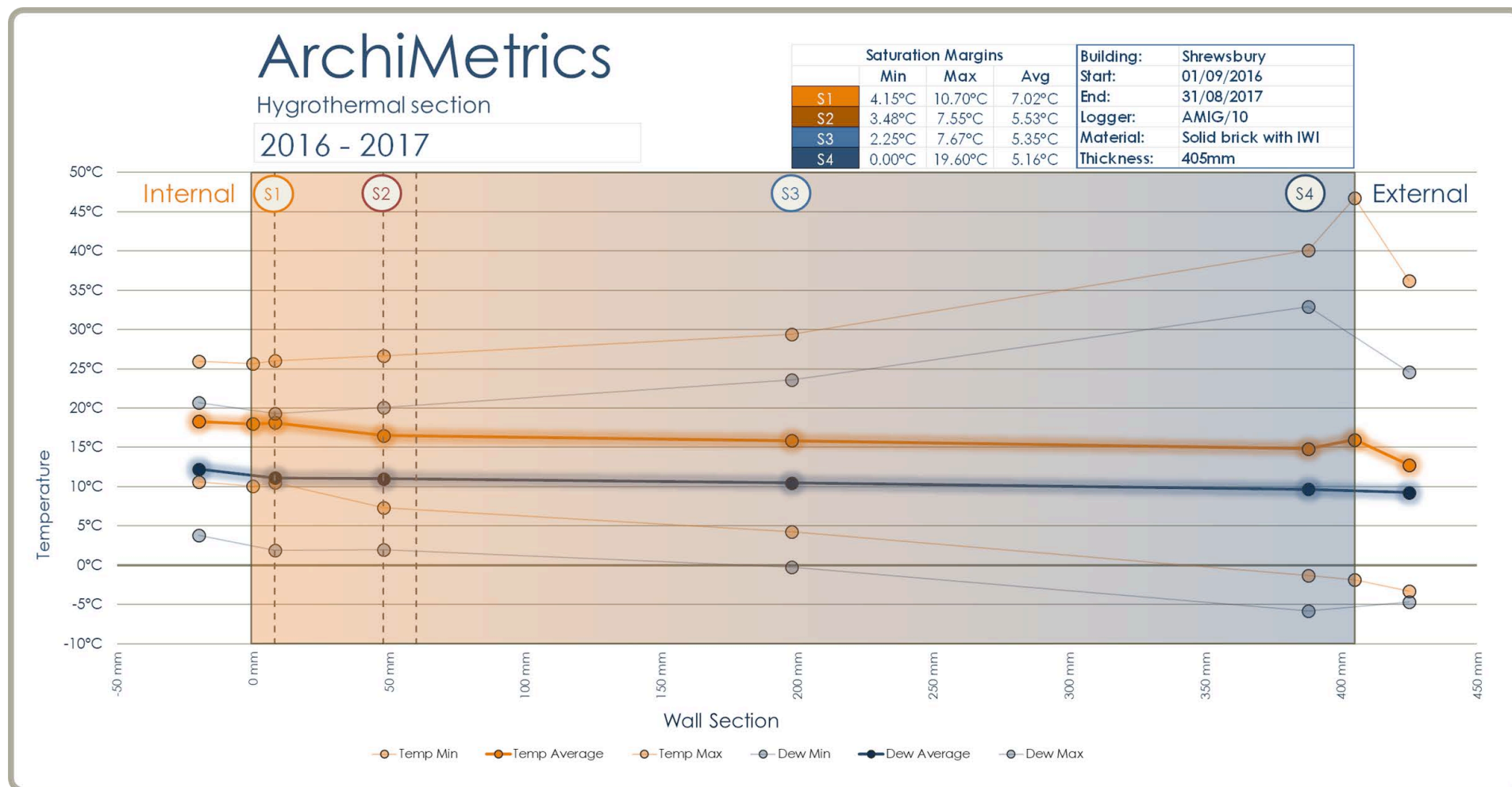
Figure 12. Hygrothermal section, Abbeyforegate, Shrewsbury 2016–2017 (capped).
