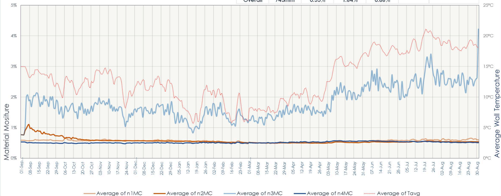
Figure 34. Material moisture content over time, Mill House, Drewsteignton, 2015-2016.
