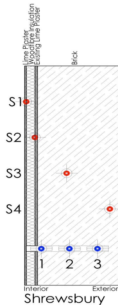
Figure 4. Position of wall sensors through section, Shrewsbury – red IHGM, blue material moisture.
