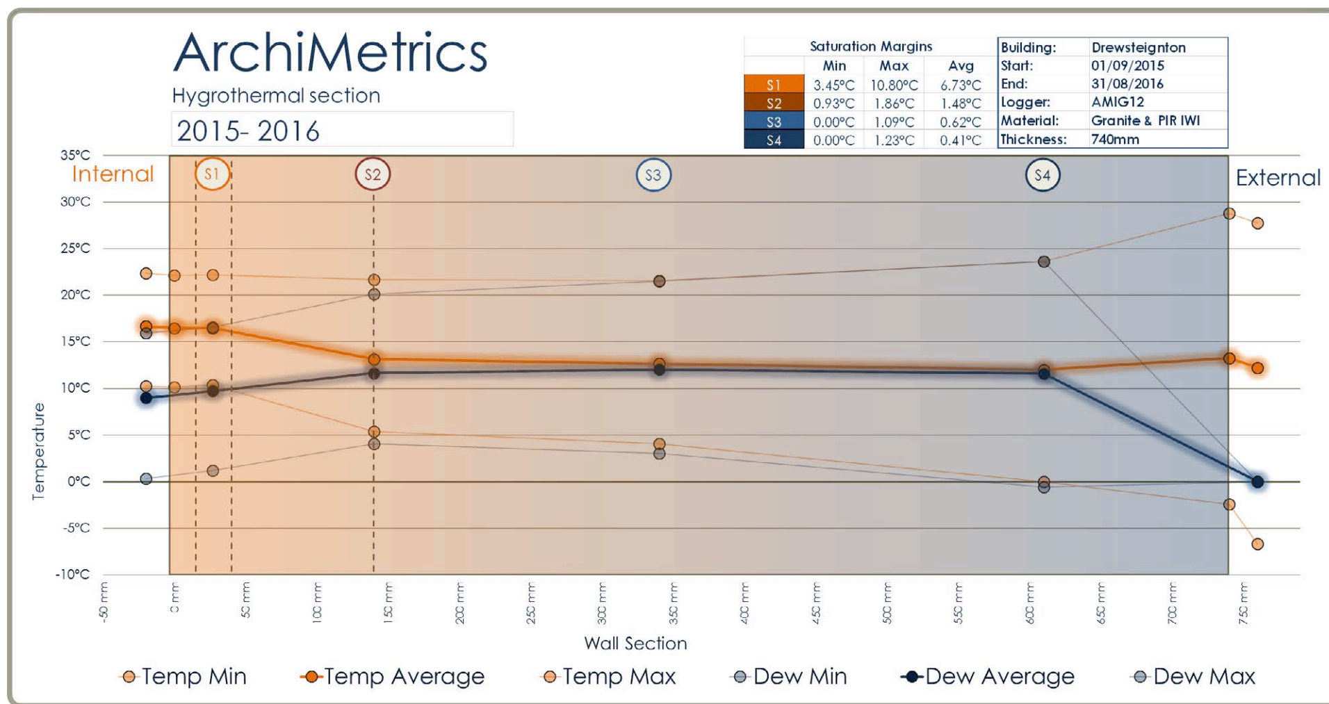
Figure 29. Hygrothermal section, Mill House, Drewsteignton, 2015–2016 (capped).
