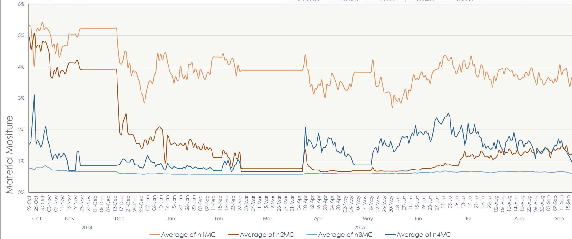
Figure 48. Material moisture content over time, The Firs, Riddlecombe 2014-2015
