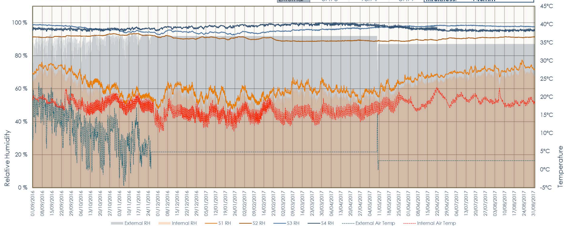
Figure 24. Relative humidity over time, full resolution, Mill House, Drewsteignton, 2016-2017.
