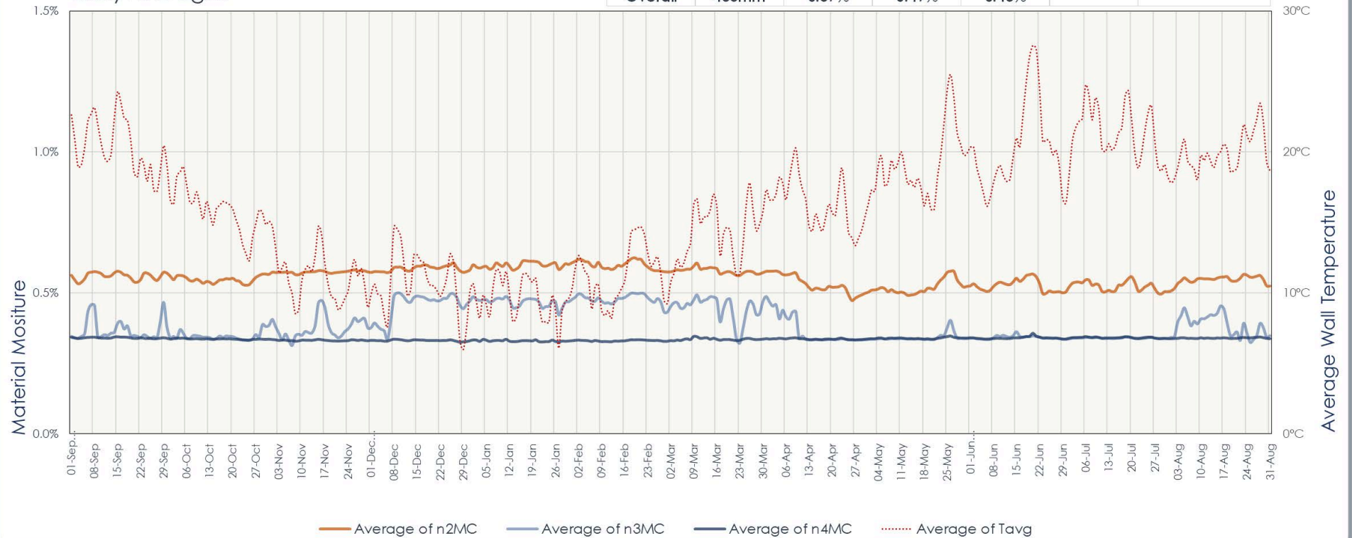
Figure 17. Material moisture content over time, Abbeyforegate, Shrewsbury 2016-2017.
