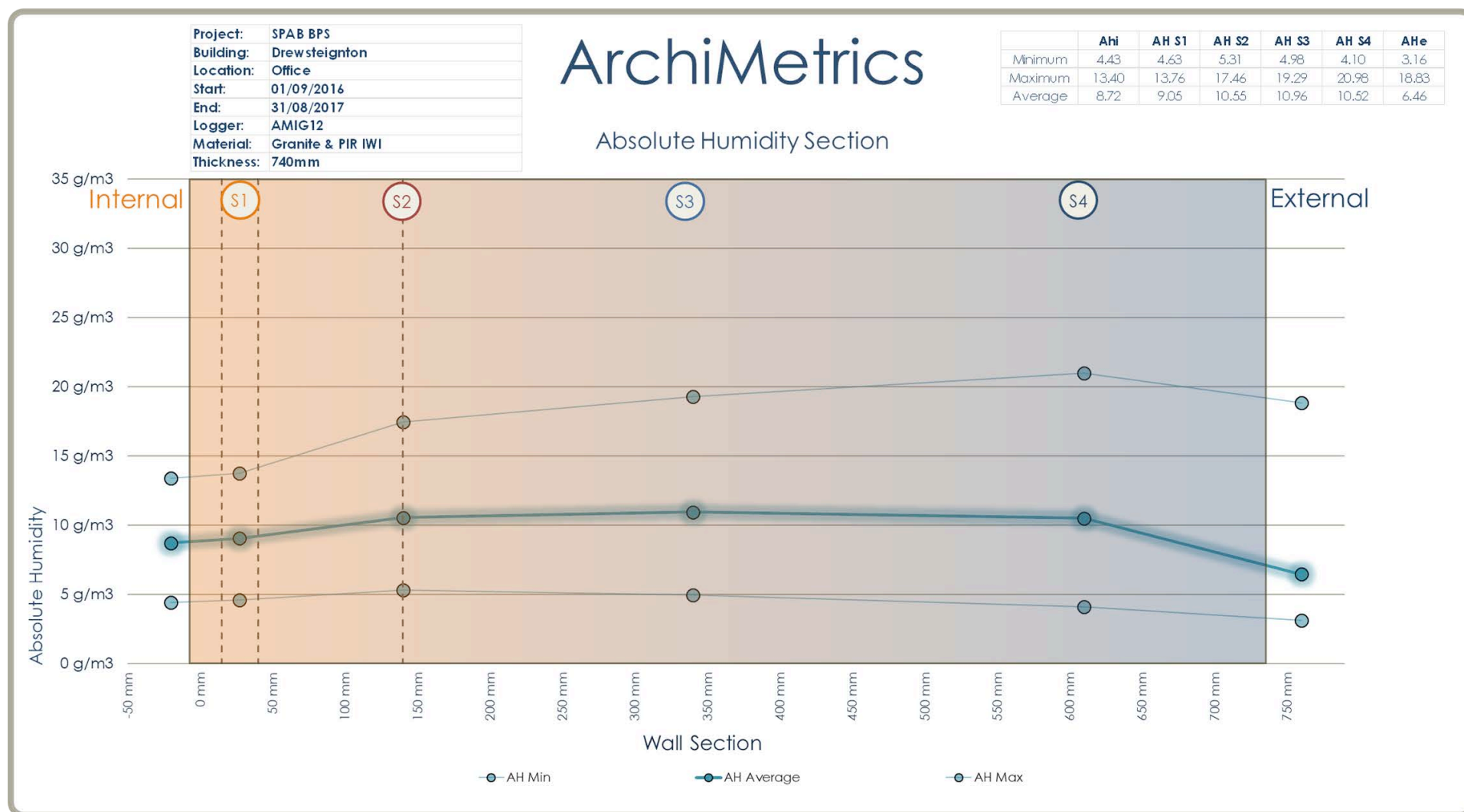
Figure 54. Absolute humidity average section, Drewsteignton, 2016-2017.
