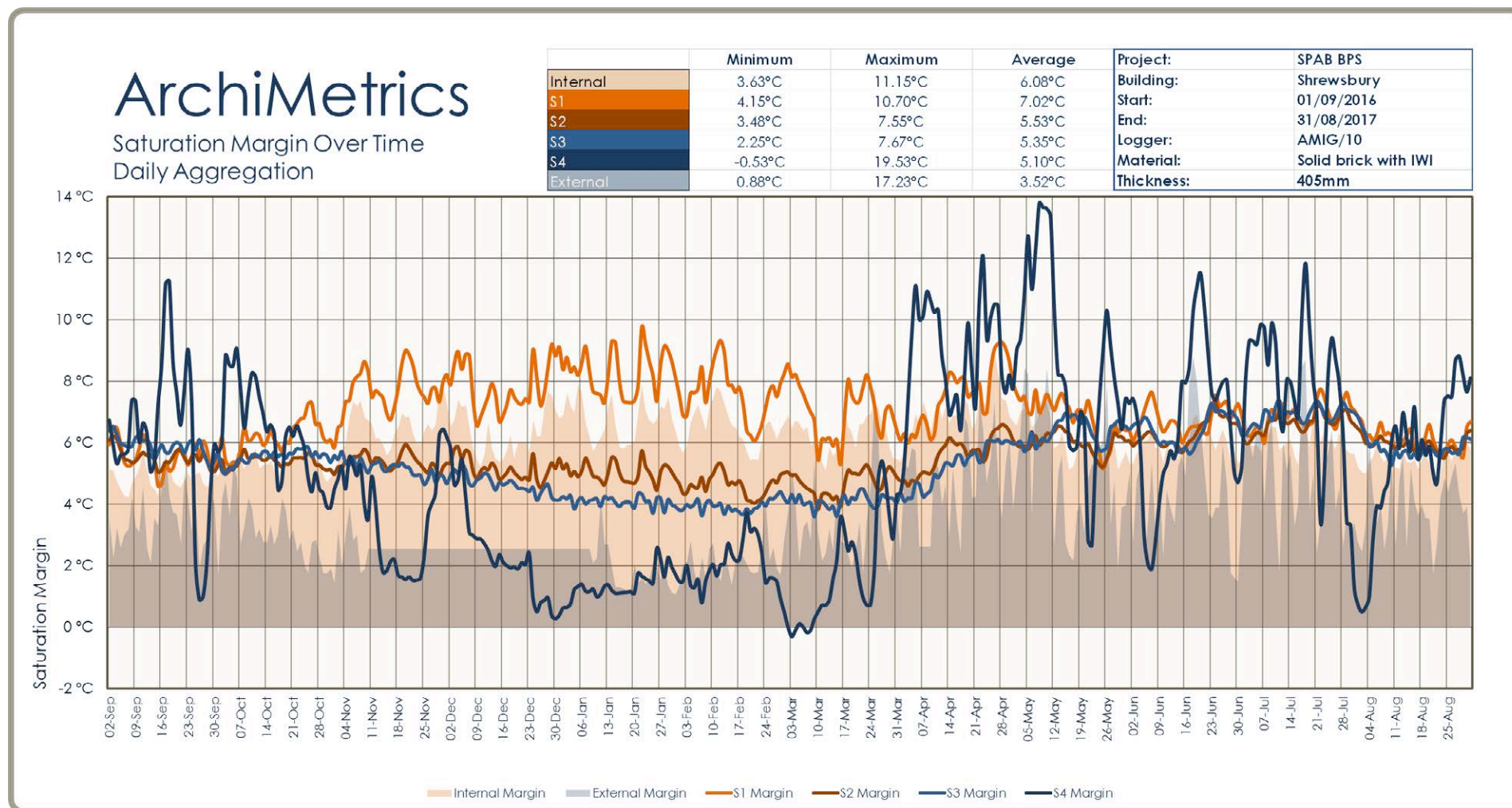
Figure 11. Saturation margin over time, Abbeyforegate, Shrewsbury 2016-2017.
