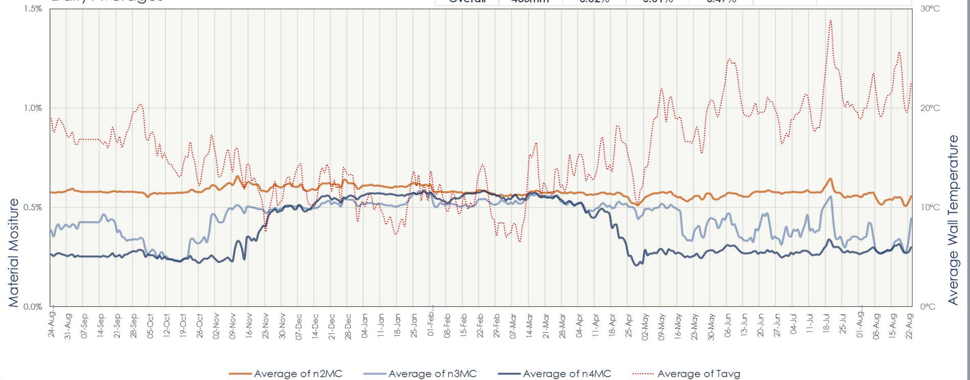
Figure 18. Material moisture content over time, Abbeyforegate, Shrewsbury 2015-2016.
