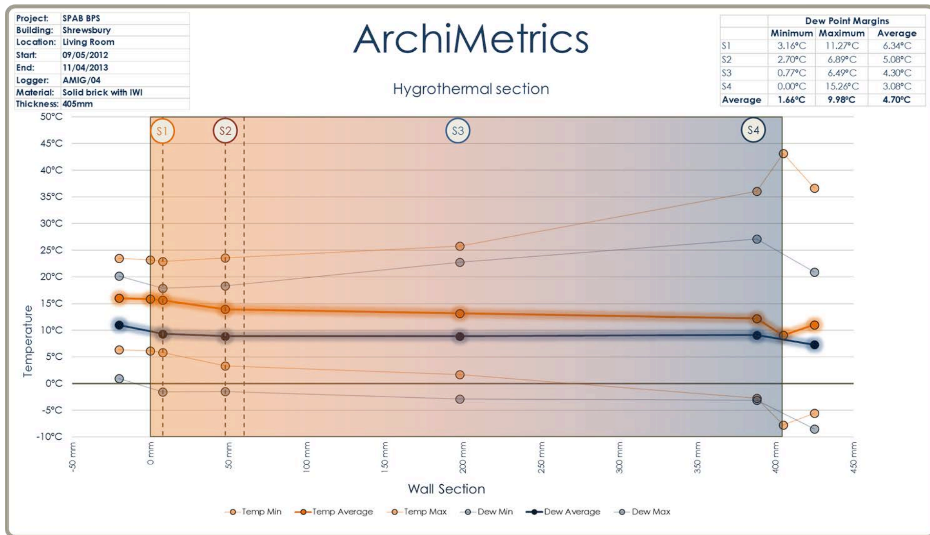
Figure 16. Hygrothermal section, Abbeyforegate, Shrewsbury, 2012-2013.
