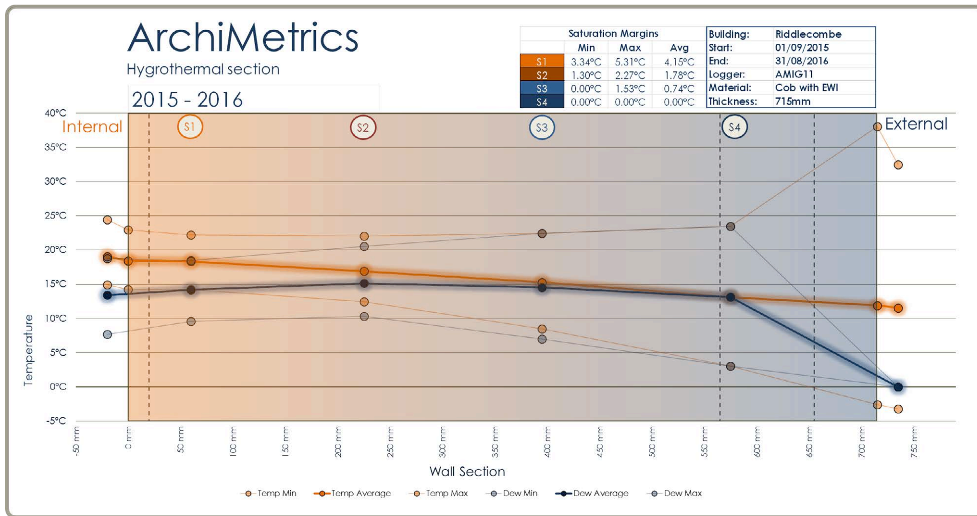
Figure 43. Hygrothermal section, The Firs, Riddlecombe, 2015-2016.
